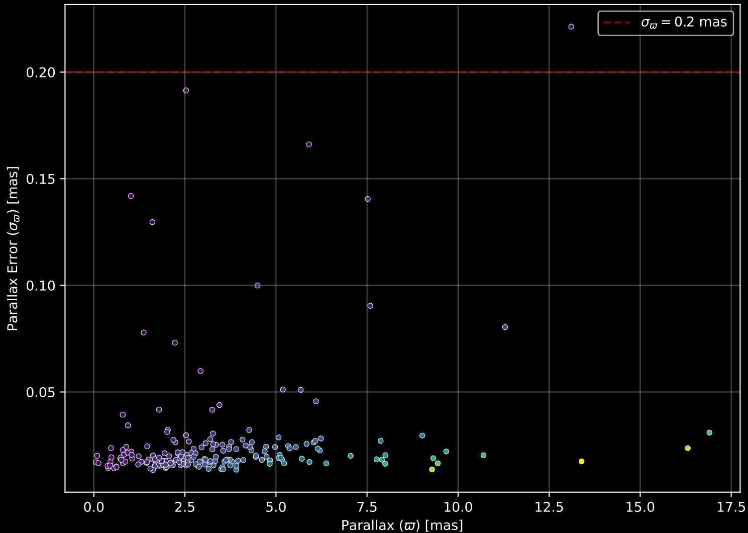
APOGEE DR17 Field: [049+90_MGA] Parallax Quality (n= 192)
