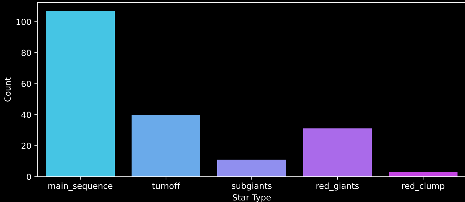
APOGEE DR17 Field: [049+90_MGA] Count plot of Star Type
