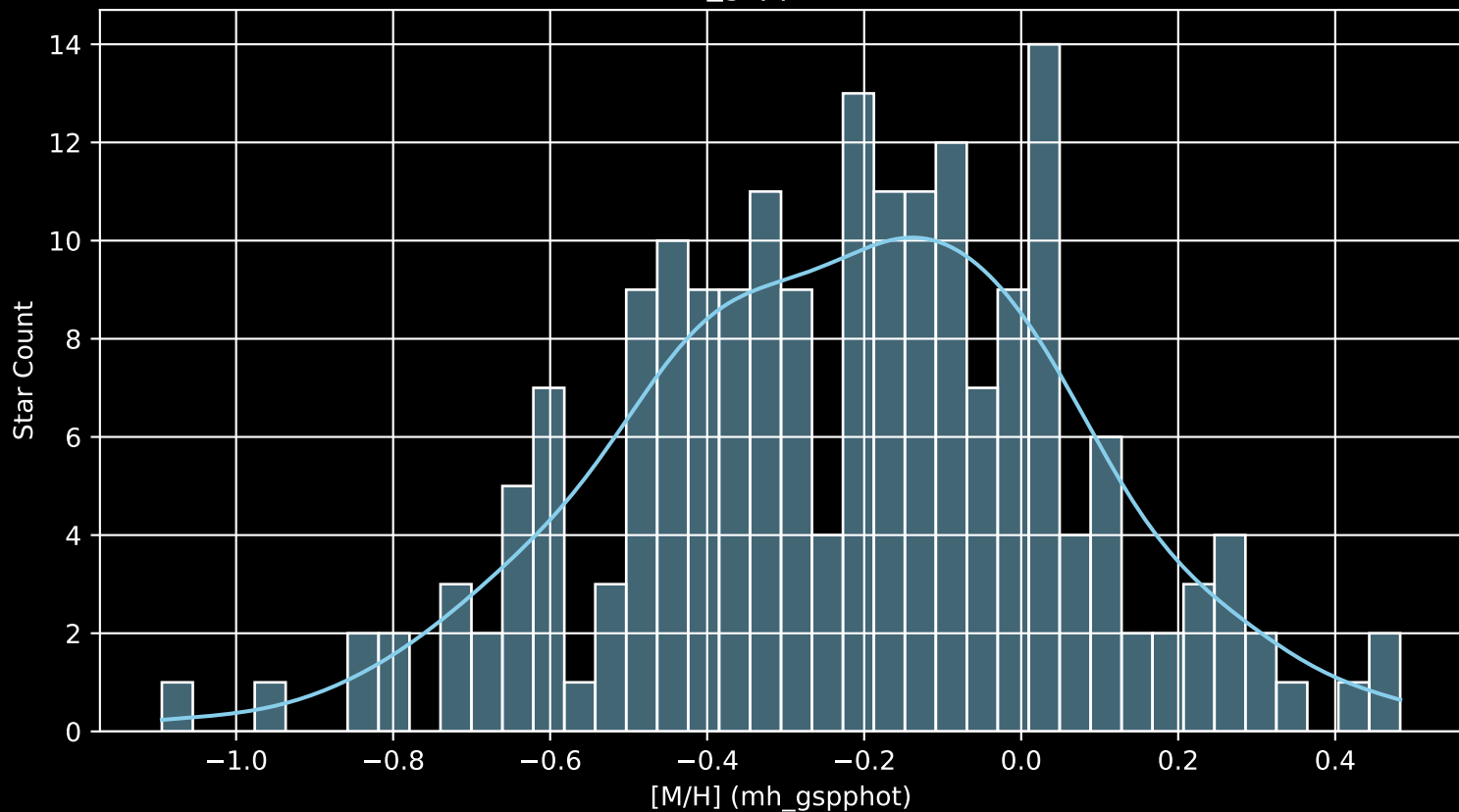
APOGEE DR17 Field: [049+90_MGA [M/H] (mh_gspphot) (n= 192)
