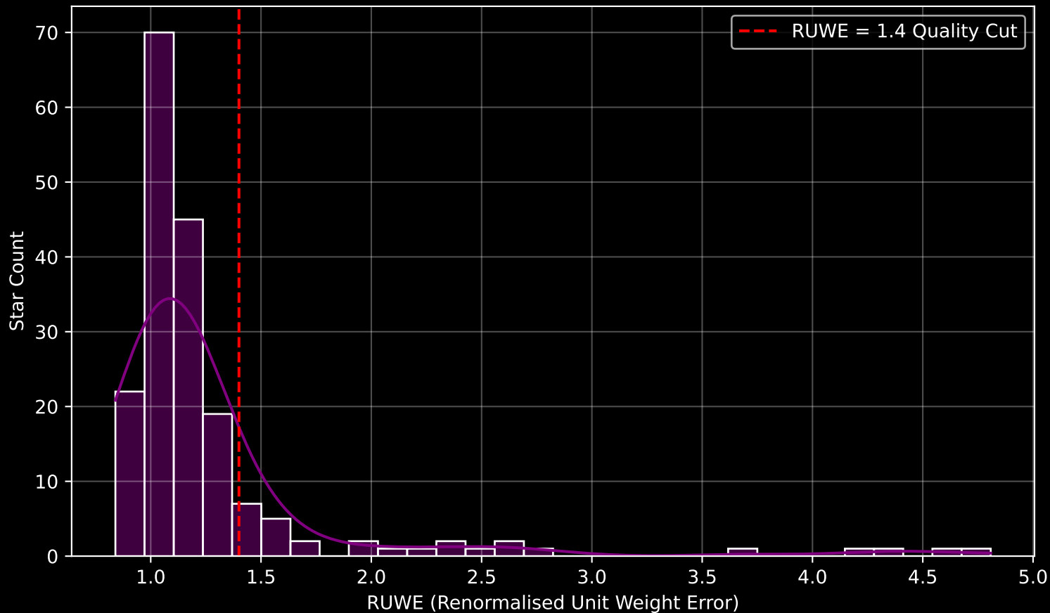
GAPOGEE DR17 Field [049+90_MGA] RUWE Distribution (n= 185)
