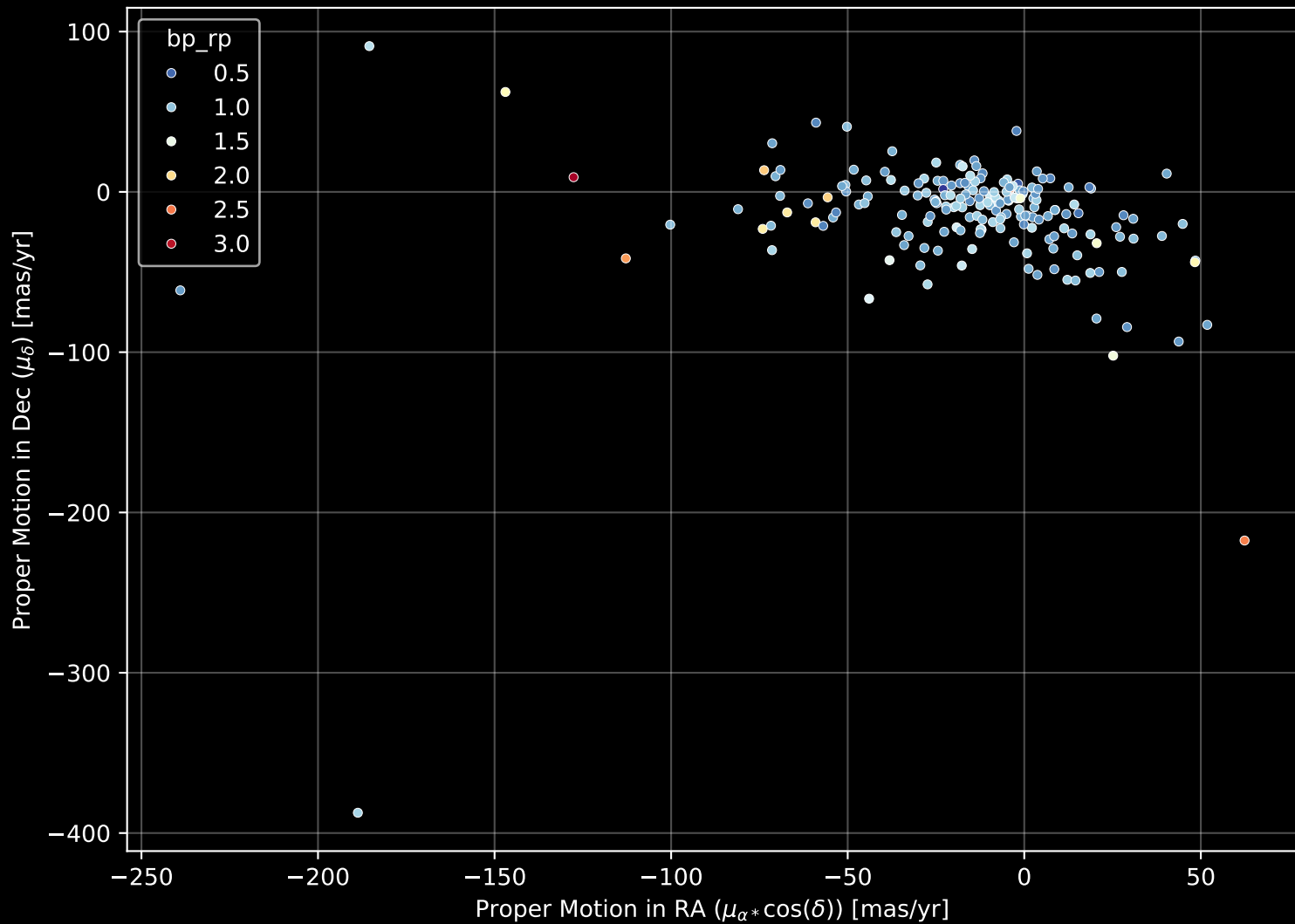
APOGEE DR17 Field: [049+90_MGA] Proper Motion Diagram (n= 192)
