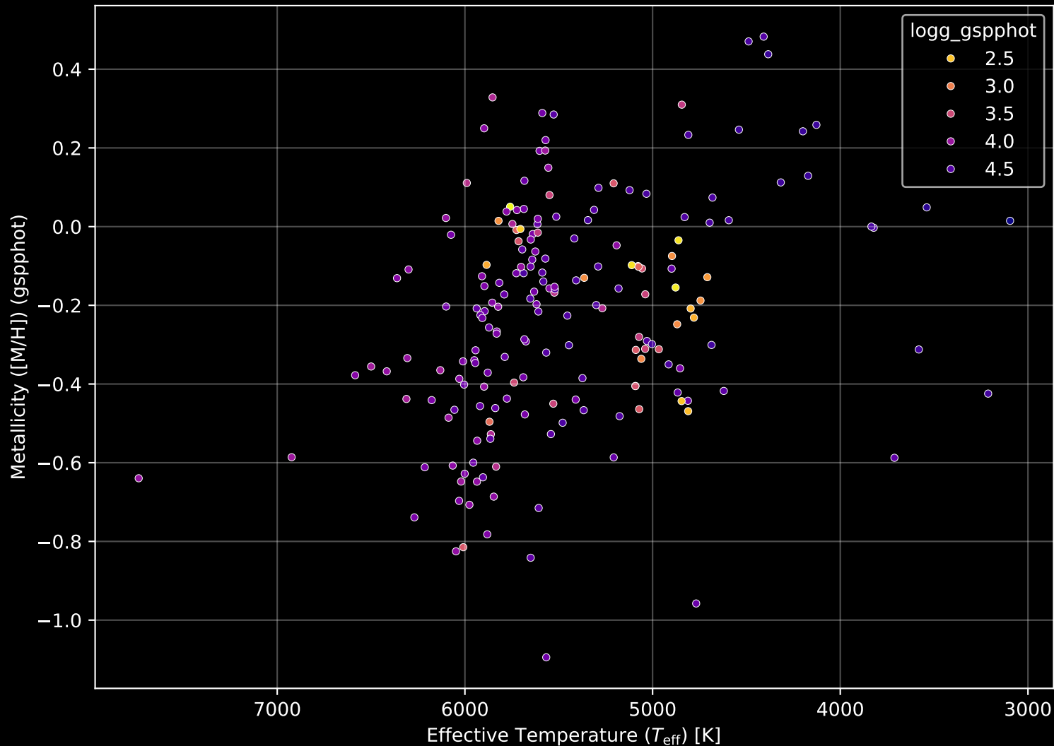
APOGEE DR17 Field: [049+90_MGA] Stellar Population Parameters (n= 192)
