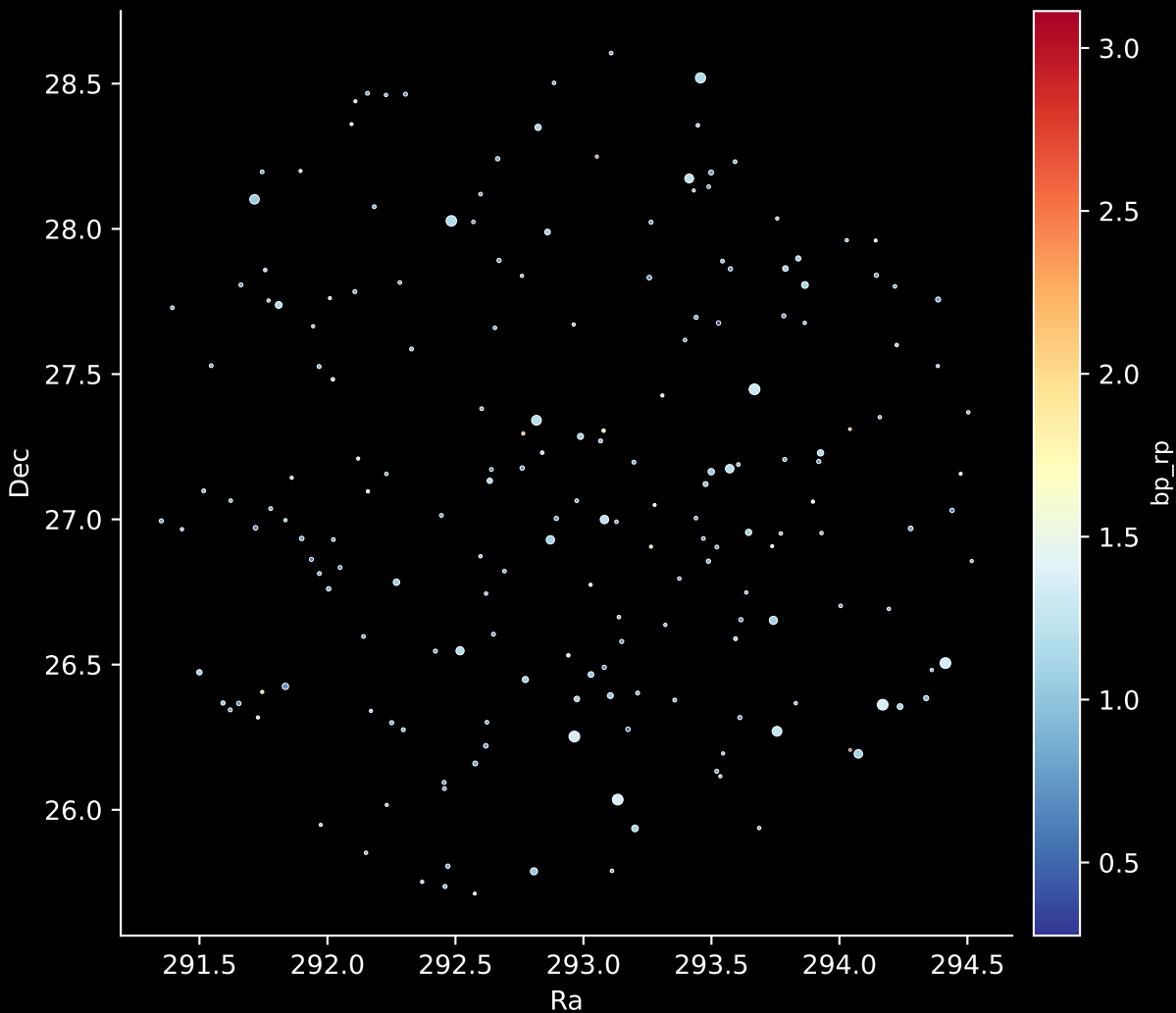
APOGEE DR17 Field: [049+90_MGA] Stars: 192
